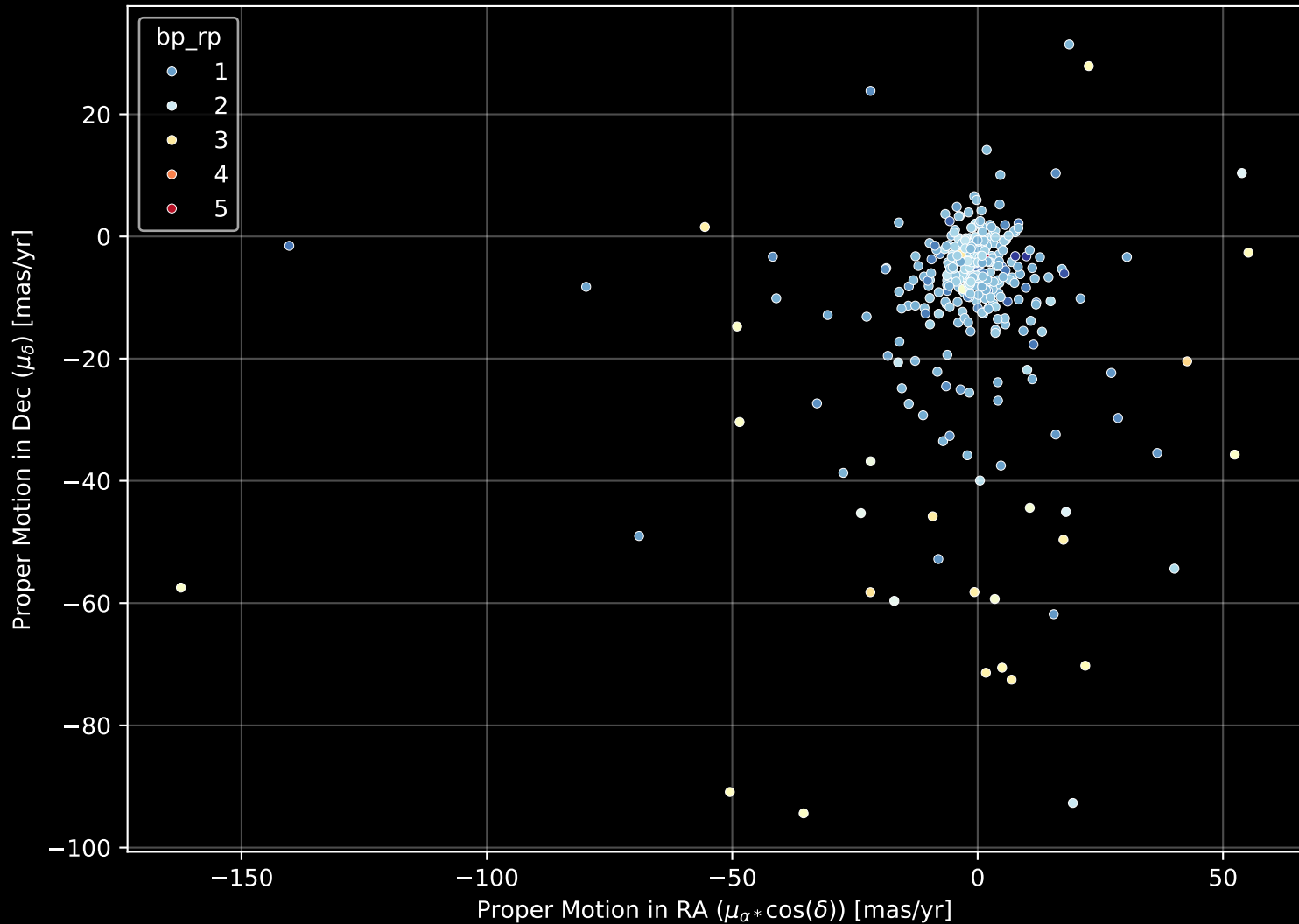
APOGEE DR17 Field: [K2_C7_009-18] Proper Motion Diagram (n= 366)
