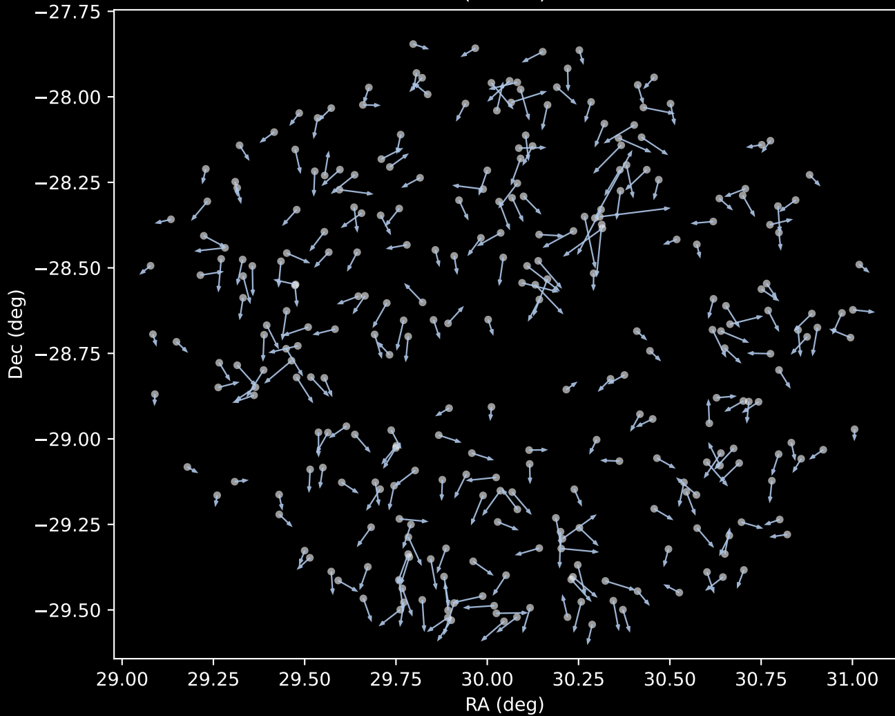
APOGEE DR17 Cluster 1 Proper Motion Vectors (n=293)
