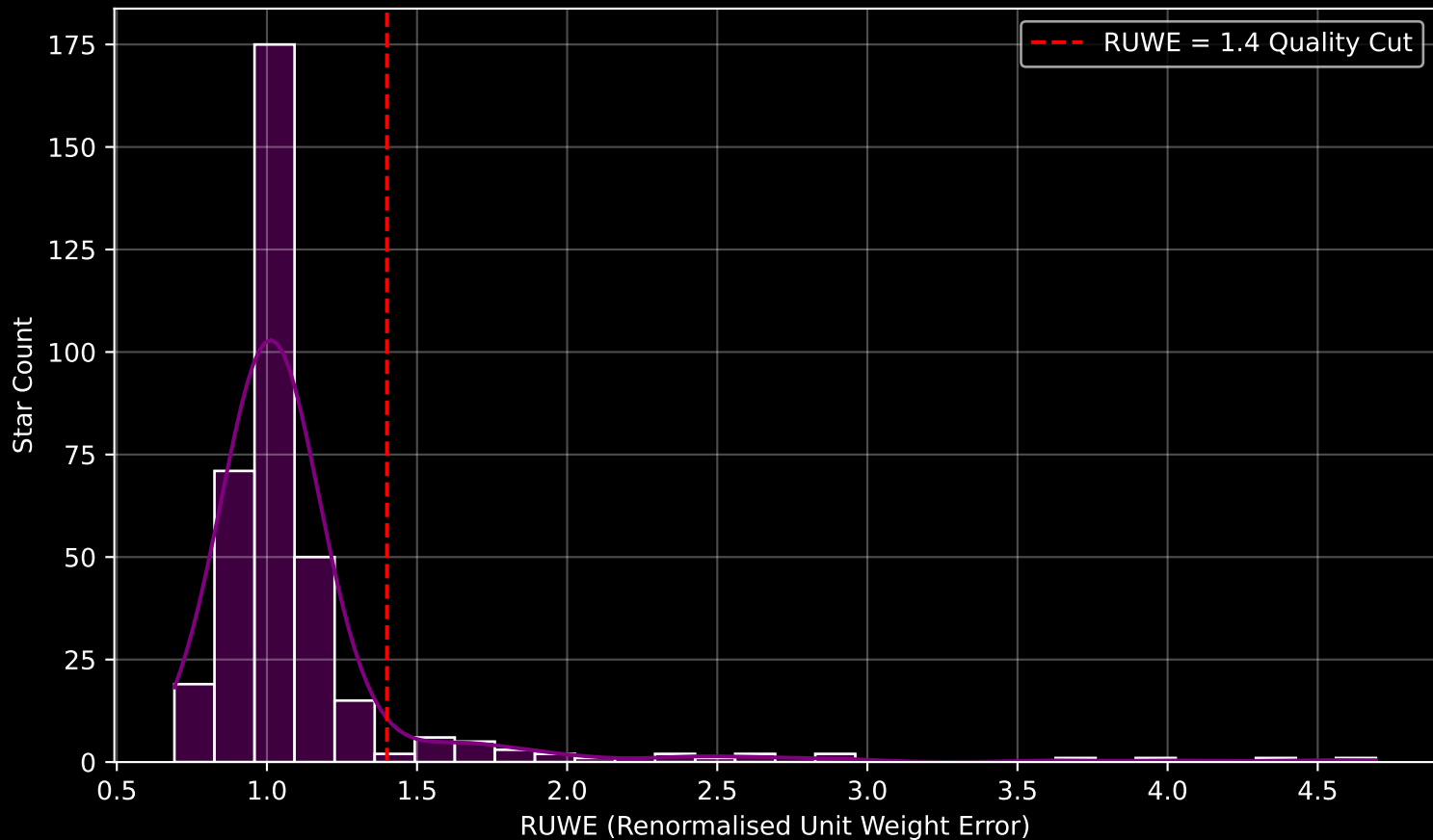
GAPOGEE DR17 Field [K2_C7_009-18] RUWE Distribution (n= 360)
