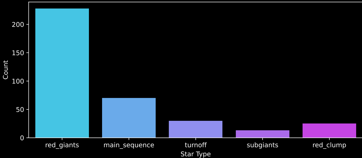
APOGEE DR17 Field: [K2_C7_009-18] Count plot of Star Type
