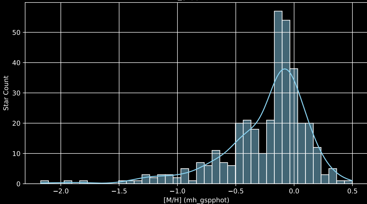
APOGEE DR17 Field: [K2_C7_009-18 [M/H] (mh_gspphot) (n= 363)
