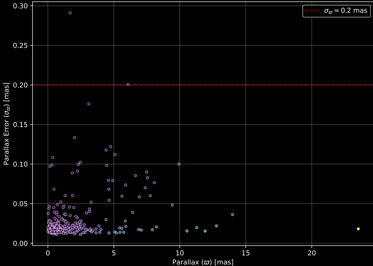
APOGEE DR17 Field: [K2_C7_009-18] Parallax Quality (n= 366)
